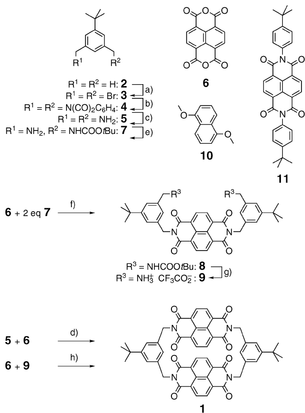
Scheme 1 Synthesis of the macrocycle 1 and its precursors. † Molecular structures of the compounds 10 and 11 . (a) NBS, AIBN, CH_3CO_2H , h\nu , 4.5 h, 48%; (b) C_6H_4(CO)_2NK , K_2CO_3 , CH_3CN , reflux, 5 h, 86%; (c) N_2H_4 , MeOH, reflux, 2 h, 82%; (d) Et_3N , i -PrOH, reflux, 3 d, 2–3%; (e) BOC_2O , CHCl_3 , 0 °C, 5 h, 47%; (f) Et_3N , i -PrOH, reflux, 3 d, 44%; (g) CF_3COOH , CH_2Cl_2 , rt, 2 h, 100%; (h) Et_3N , i -PrOH, reflux, 3 d, 40%.
